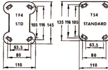
Use M10 bolts
