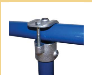
135 [Clamp-on Tee (1 bolt)] code each size 6 SCF6135 £6.55 size 8 SCF8135 £9.20
