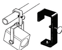
Hook Clamp
